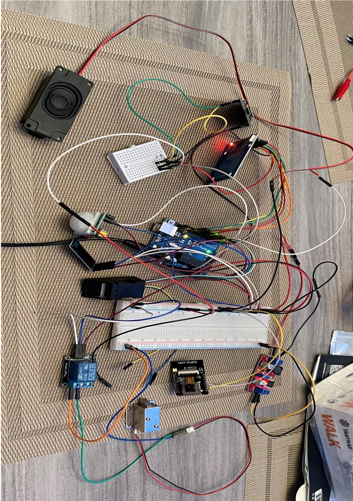
Figure 5.0: Breadboard Testing
