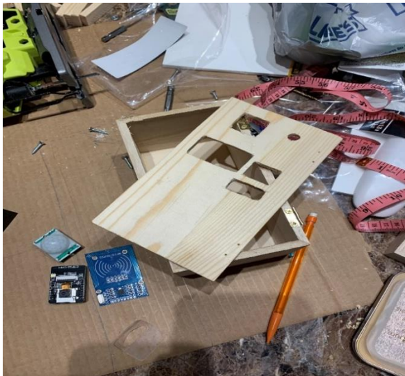
Figure 4.0: Enclosure Design
