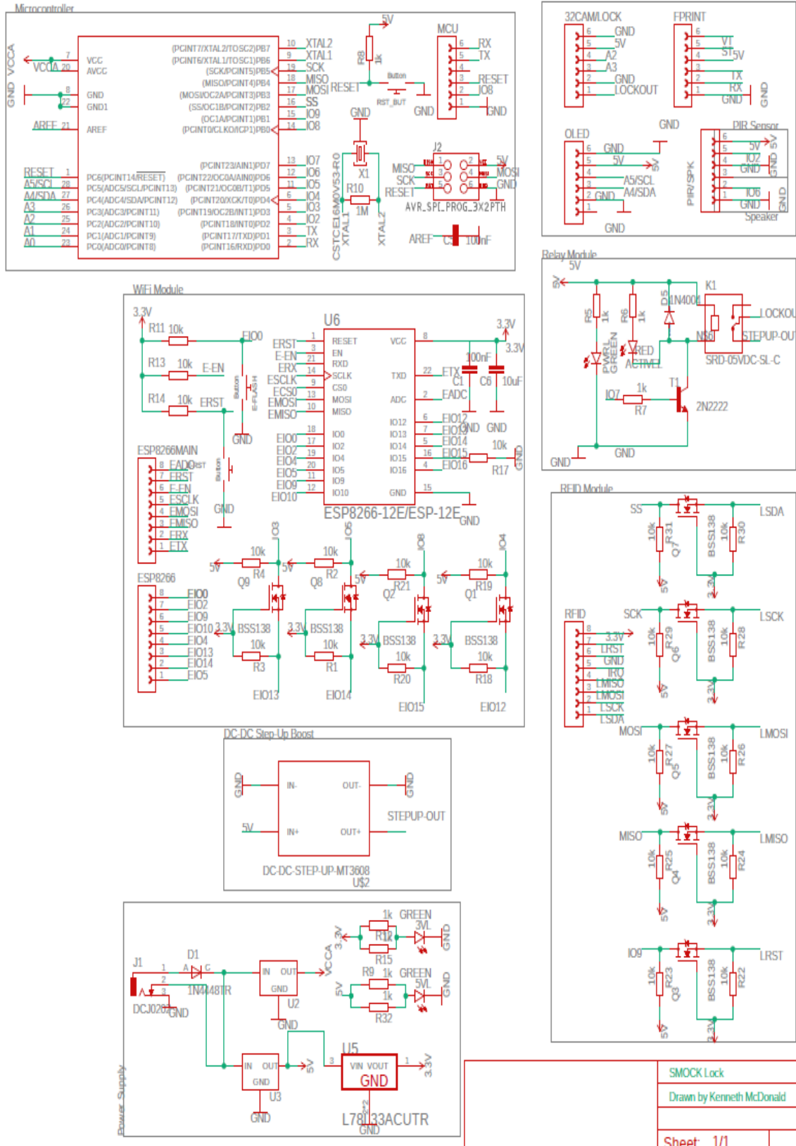
Figure 3.0: SMOCK Lock Schematic
