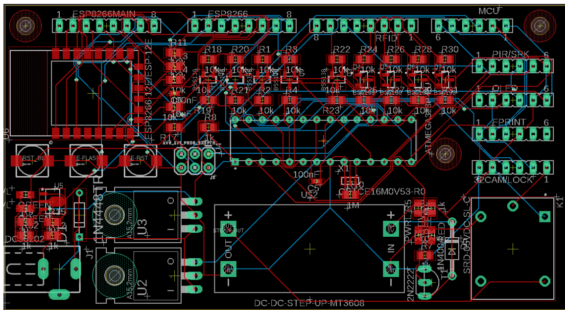
Figure 9.0 Board Design of PCB
